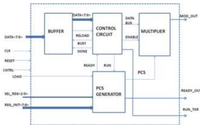
Fig.4: Block Diagram of Transmitter
