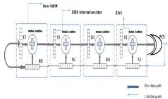
Figure 2 Block Diagram of PN Sequence Generator
