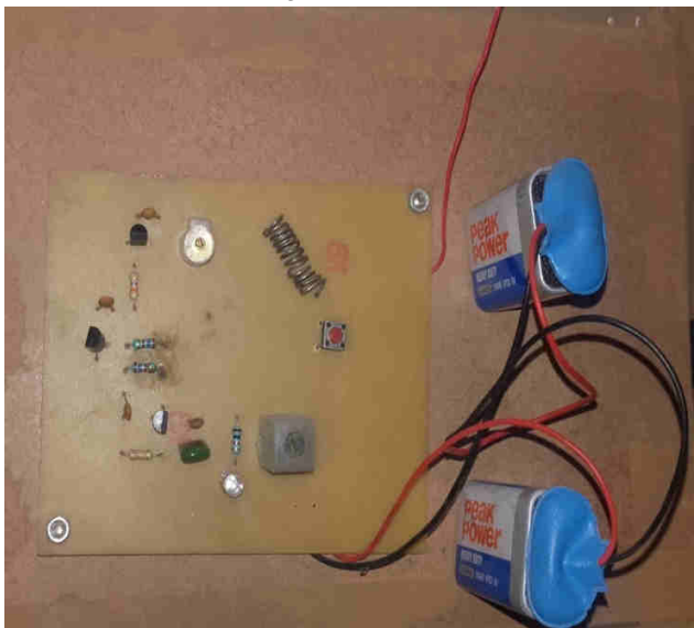
Fig. 4: Transmitter
