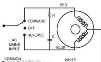
Fig. 3: Motor circuit
