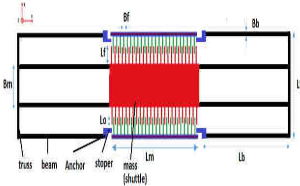
Fig.1: Schematic diagram of folded beam electrostatic energy harvester.
