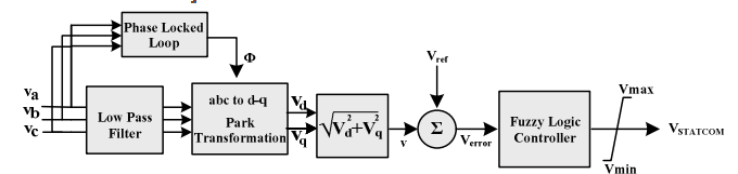
Fig.4: Block diagram for STATCOM control system
