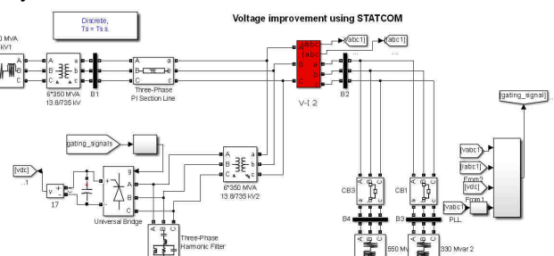
Fig.6: System model for simulation
