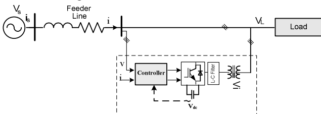
Fig.3: Fundamental connection of STATCOM
