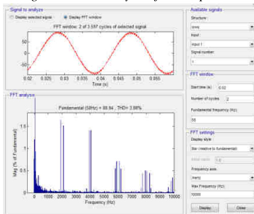
Fig.9: Fourier analysis of the line current after STATCOM voltage injected
