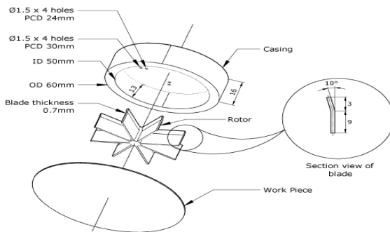
Fig.2: Design dimensions
