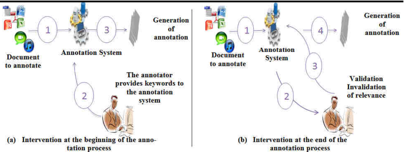
Fig.1: Semi-Automatic Annotation
