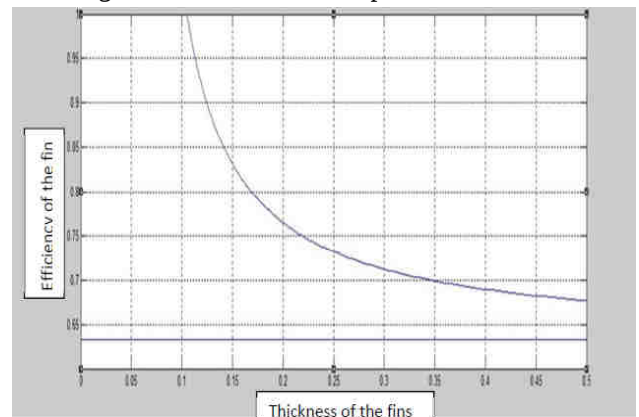
Fig. 10: Thickness of the fins / Efficiency of the fins 13
