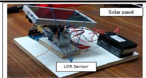
Fig. 4: Complete Hardware assembly
