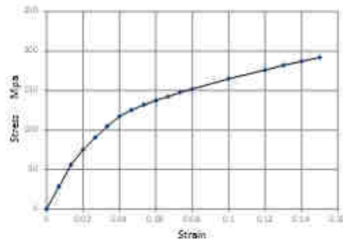
Fig. 3: Stress-strain curve of Torlon 4203L
