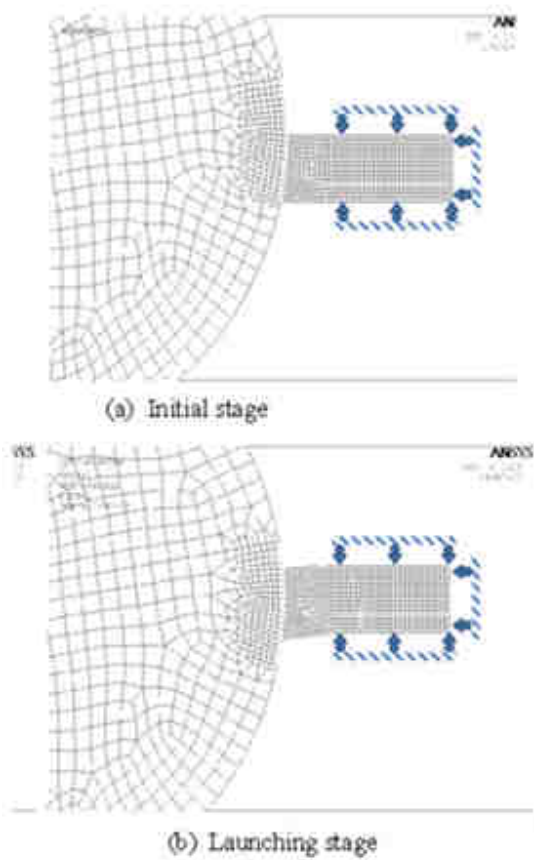
Fig.4: Deformation of a projectile trap at launching stage
