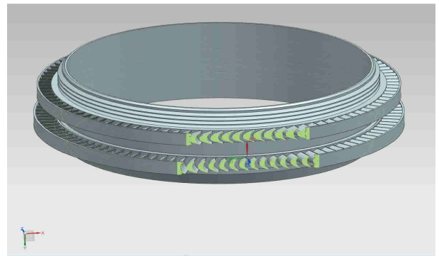
Fig.1: LPOT Turbine rotor modeled in NX CAD
