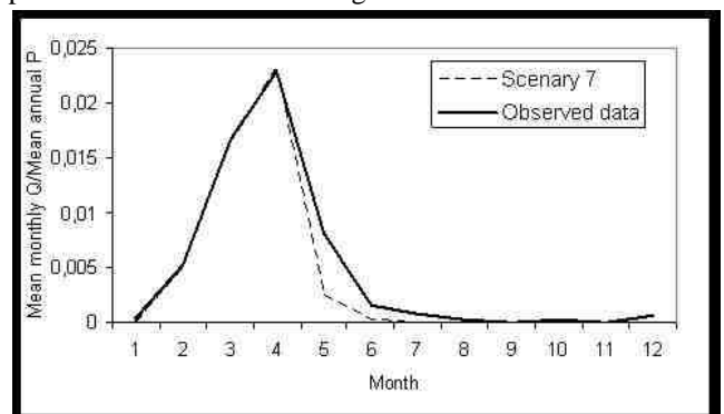
Fig.19: Comparison of observed and estimated monthly surface runoff by refined model in Taperoa river, Poco de Pedras sub-basin.
