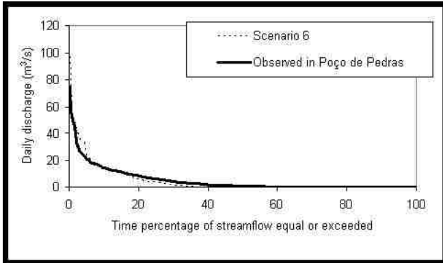
Fig.26: Daily flow duration curve observed and estimated by refined model in Taperoa river.
