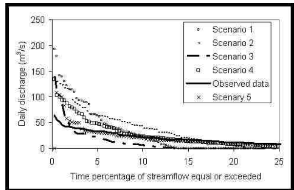
Fig.10: Curves duration of flow observed and estimated by refined model daily, in Paraiba river, Caraubas sub-basin.
