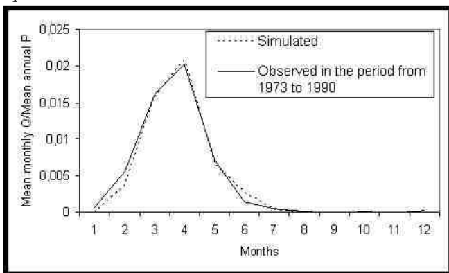
Fig.27: Monthly runoff observed and estimated for refined model in Epitacio Pessoa basin.
