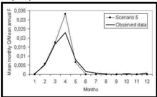
Fig.17: Comparison of monthly surface runoff estimated and observed by model refined in Taperoa river, Poco de Pedras sub-basin.
