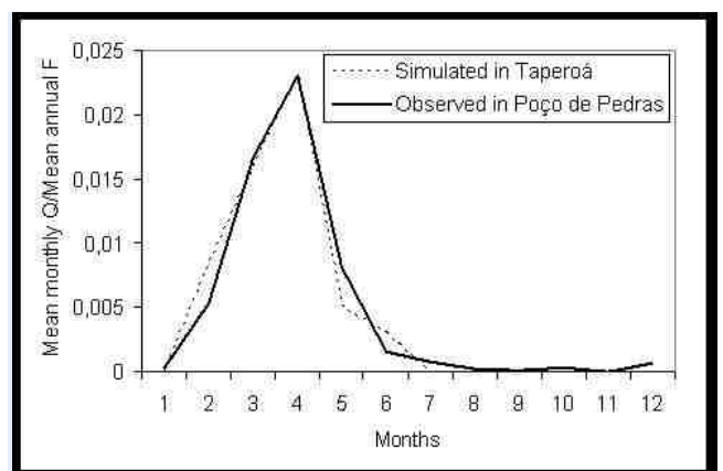
Fig.25: Runoff observed and estimated monthly by refined model in Taperoa Sub-basin.
