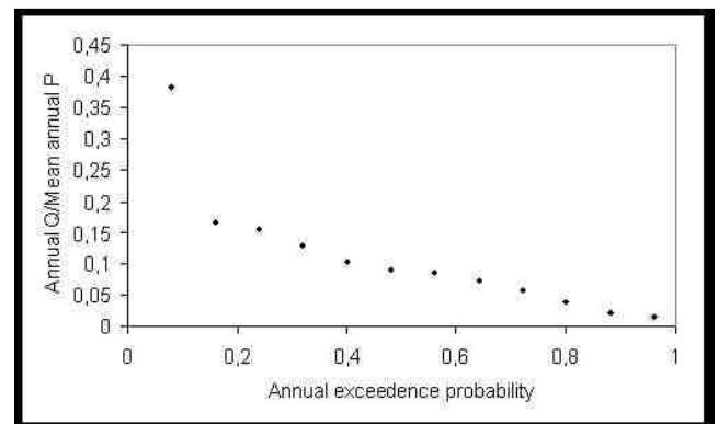
Fig.29: Estimated annual runoff estimated by model for Epitacio Pessoa basin.
