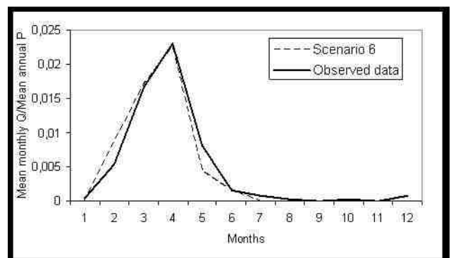
Fig.18: Comparison of monthly surface runoff estimated and observed by refined model in Taperoa river, Poco de Pedras sub-basin.
