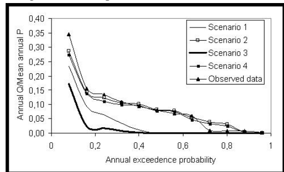
Fig.3: Probability surplus of the observed superficial runoff and estimated by the annual model in Caraúbas Monthly water balance
