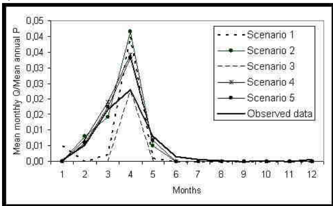
Fig.16: Comparison of monthly surface runoff observed and estimated by model refined in Taperoa river, Poco de Pedras sub-basin.
