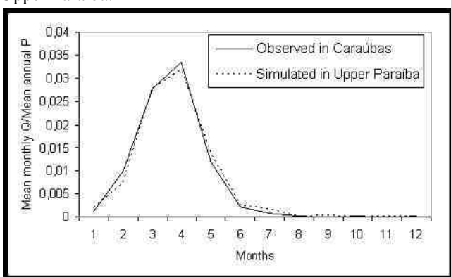
Fig.23: Runoff monthly observed and estimated by refined model in Upper Paraíba, in Caraubas sub-basin.
