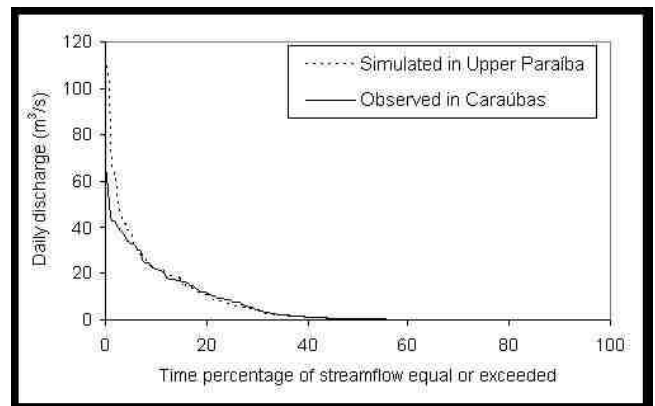
Fig.24: Duration curve of daily flows observed and estimated by refined model in Upper Paraíba, Caraubas sub-basin.
