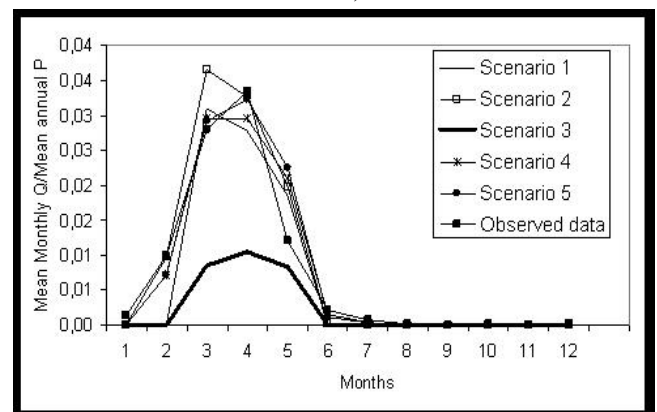
Fig.7: Comparison of monthly surface runoff observed and estimated by model refined in sub-absin of Paraíba river in Caraubas.
