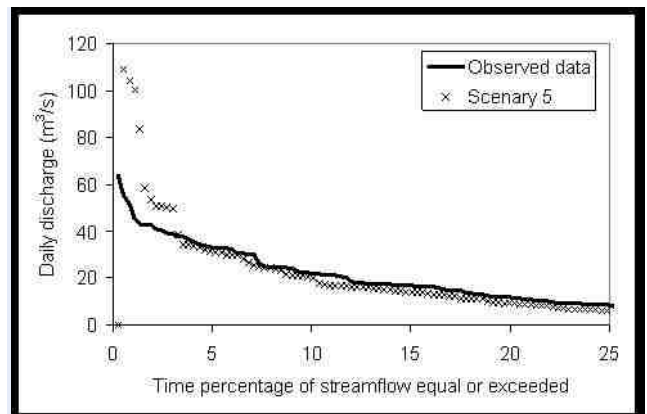
Fig.11: Curves duration of flow observed and estimated by refined model daily, in Paraiba river, Caraubas sub-basin.
