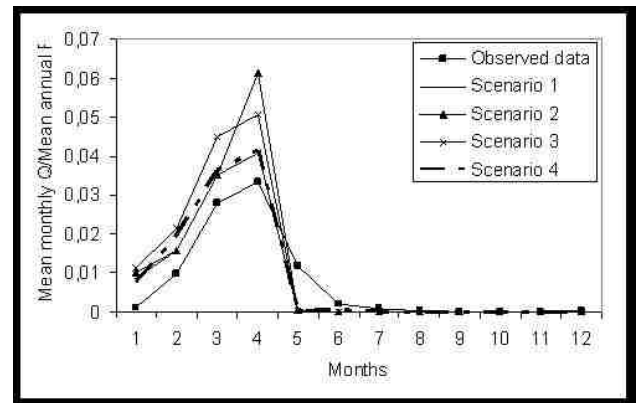
Fig.14: Comparison of monthly surface runoff observed and estimated by model in Taperoa river, Peco de Pedras sub-basin.
