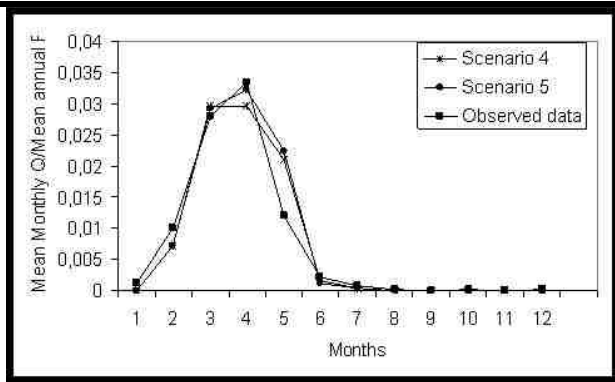
Fig.8: Comparison of monthly surface runoff observed and estimated by model refined in Sub-basin of Paraiba River, in Caraubas.
