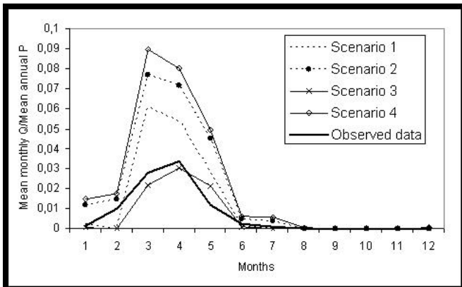
Fig.5: Comparison of surface runoff and observed monthly estimated by the model in the sub-basin of the river Paraíba, Caraúbas
