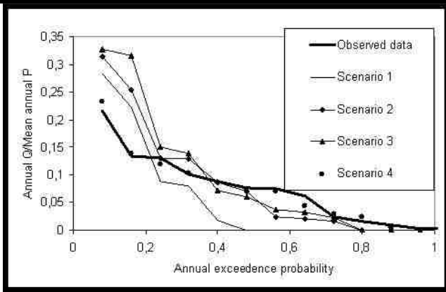
Fig.12: Probability of surplus of runoff observed and estimated by year model, in Taperoa river, Poco de Pedra sub-basin.
