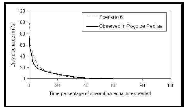
Fig.22: Curves duration of flow daily observed and estimated by refined model in Taperoa river, Poco de Pedras sub-basin.
