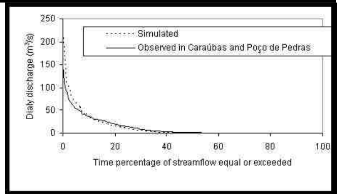
Fig.28: Daily curves duration of flow observed and estimated by refined model in Epitacio Pessoa catchment.
