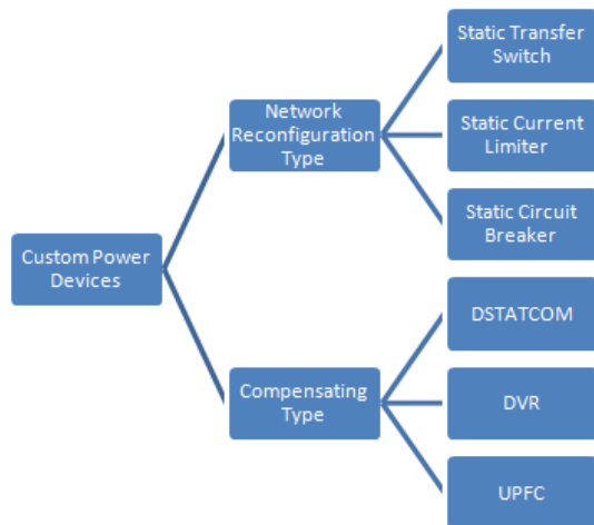
Fig.1: Configuration of custom power devices
