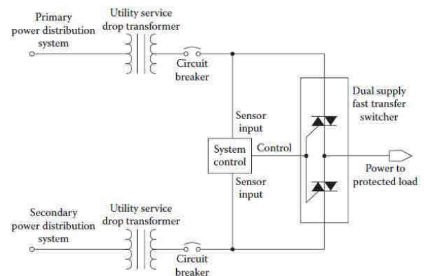
Fig.2: Static transfer Switch
