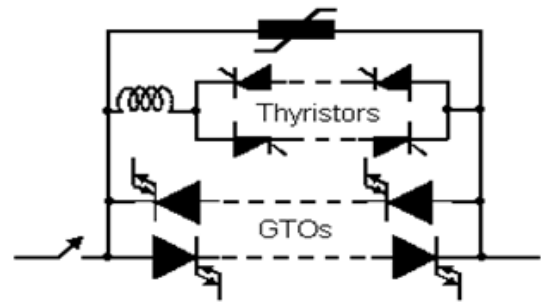
Fig.4: Static Circuit Breaker
