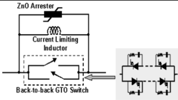
Fig.3: Static Current Limiter
