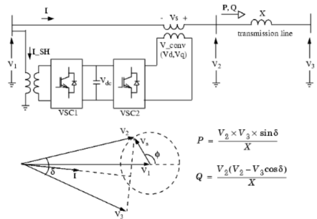
Fig.6: Block Diagram of UPFC
