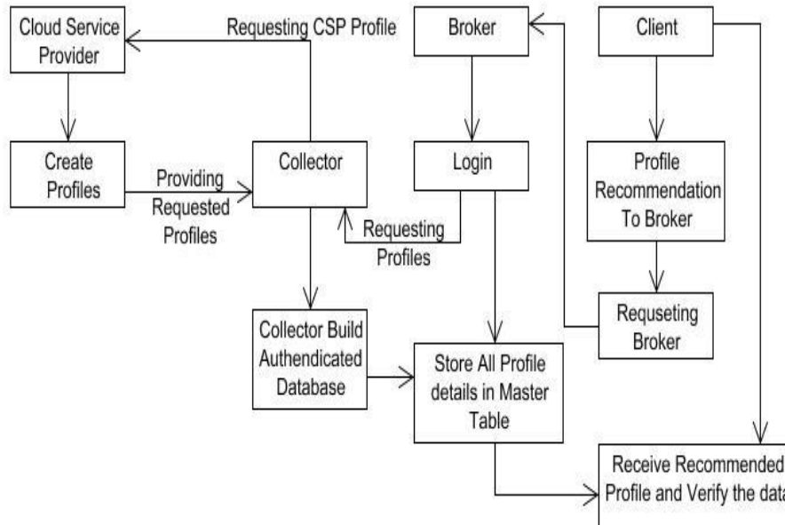
Fig.3: Work Flow Diagram for MMB-Cloud
