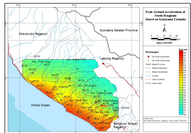
Fig.6: Distribution of peak ground acceleration value which identified in North Bengkulu based on Katayama formula calculating.
