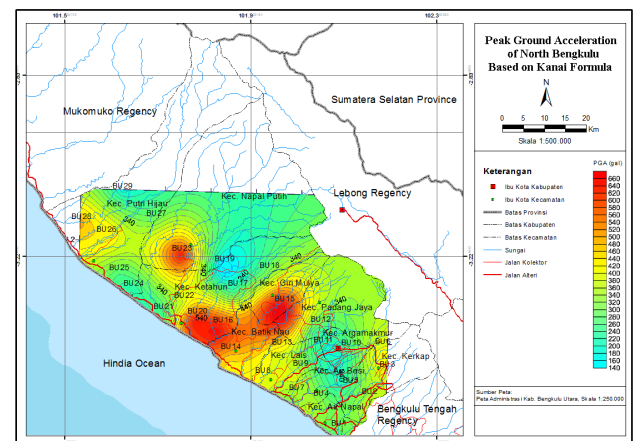
Fig.5: distribution of peak ground acceleration value which identified in North Bengkulu. this map obtained by Kanai formula calculating.
