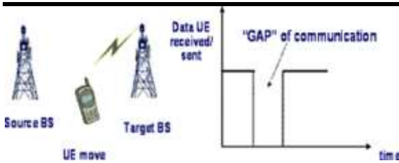
Fig.2: Hard-Handover Mechanism
