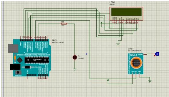
Fig 1 - Circuit Diagram
