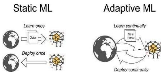
Fig2:StaticMLVsAdaptiveML
